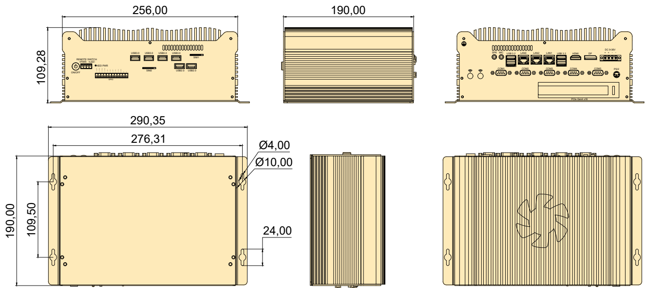
Front Panel External I/O Mechanical Layout/Drawing
