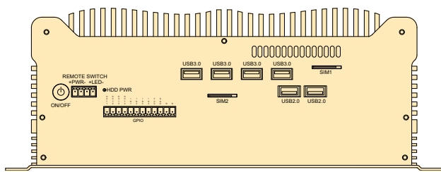
Front Panel External I/O Mechanical Layout/Drawing
