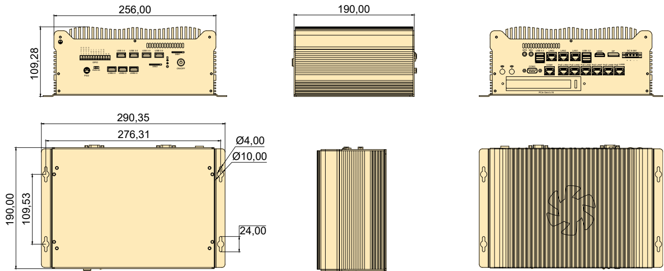
Front Panel External I/O Mechanical Layout/Drawing
