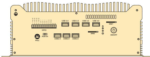
Front Panel External I/O Mechanical Layout/Drawing
