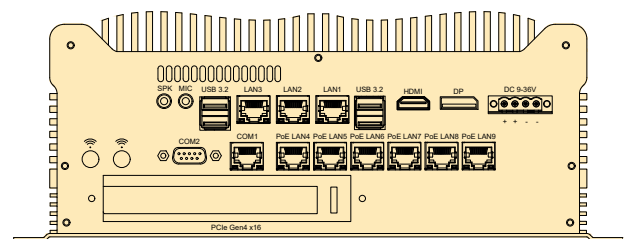
Rear Panel External I/O Mechanical Layout/Drawing
