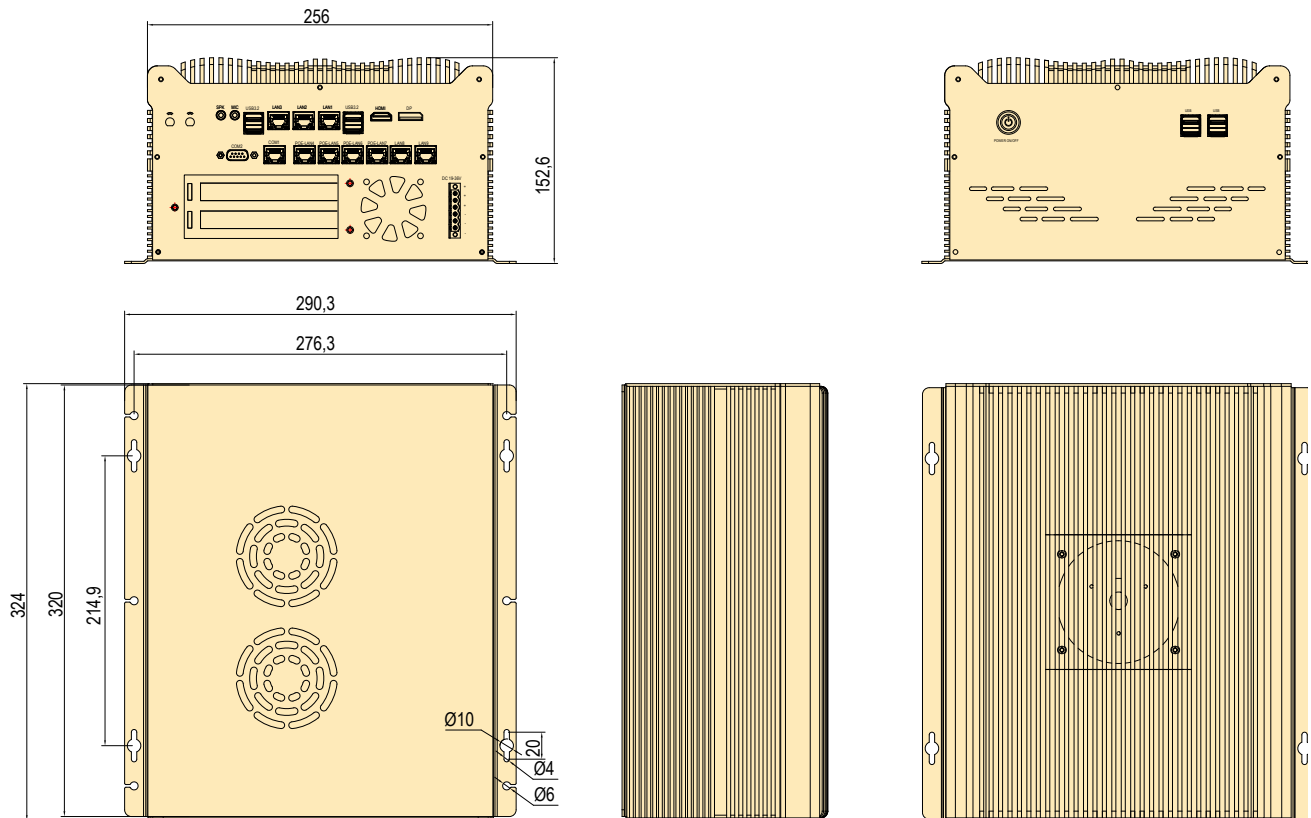
Rear Panel External I/O Mechanical Layout/Drawing
