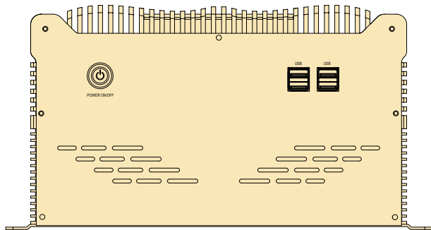
Front Panel External I/O Mechanical Layout/Drawing
